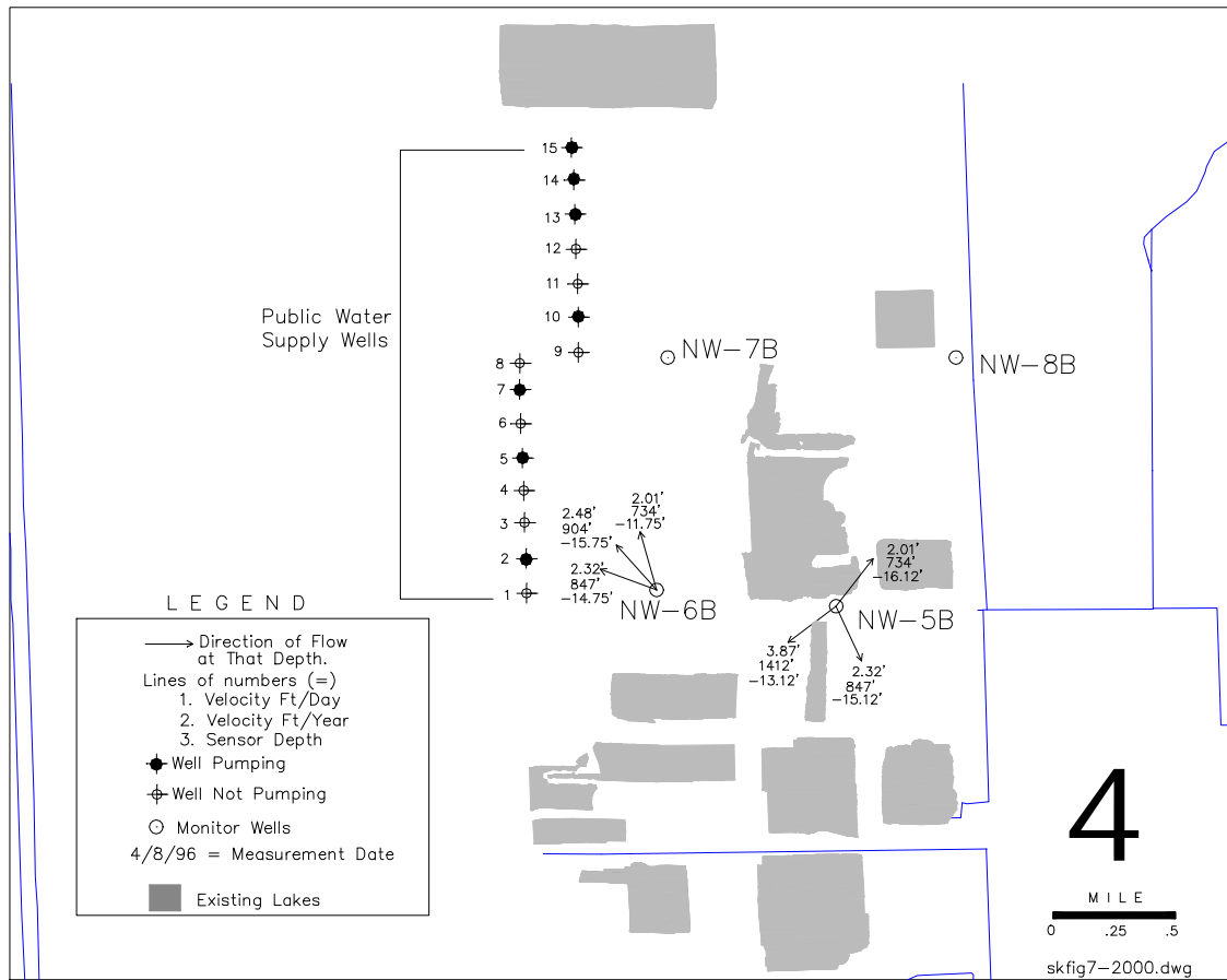
Figure 7. In situ Corrected Horizontal Groundwater Velocities in Shallow Monitor Wells at Northwest Wellfield, Miami-Dade County, Florida, April 8, 1996
